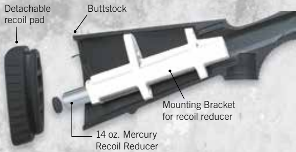
14 Item # 80208 Nova Recoil Reducer Package Includes the mercury recoil reducer and bracket for easy installaton.
